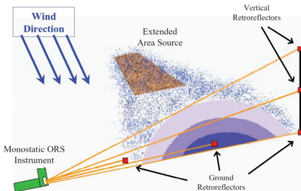
Figur 8. Radial Plume Mapping, principskiss. (20)
