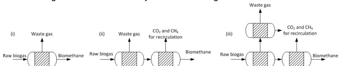
Figure 15 Three different designs of the membrane stage, that are available on the market today.
