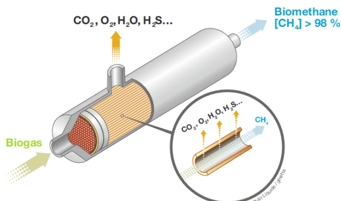
Figure 11 Illustration showing the separation involved during upgrading of biogas with membranes. Image from Air Liquide.
