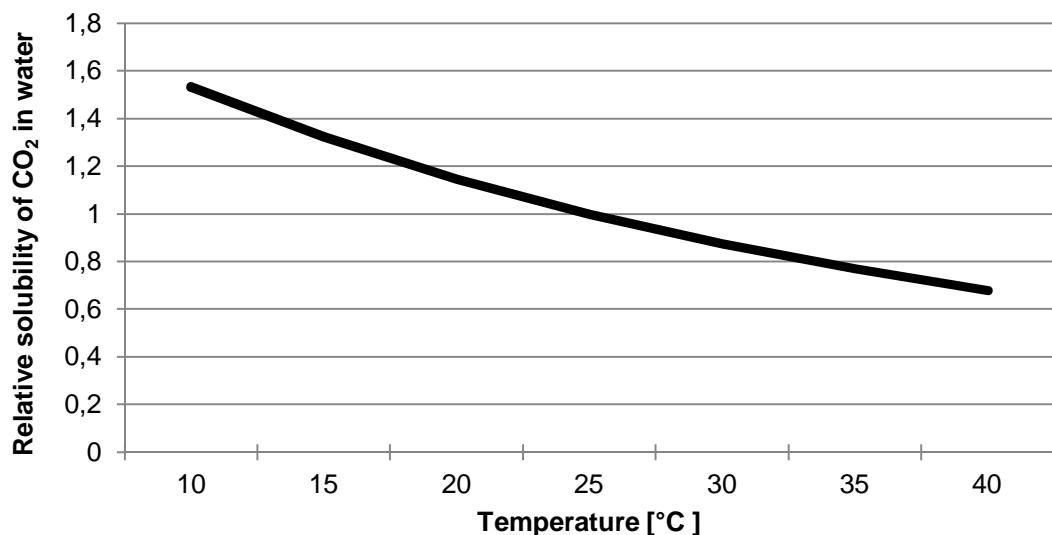
Figure 19 Relative solubility of CO_2 in water in the temperature interval between 10°C and 40°C. Solubility normalized to the value at 25°C.
